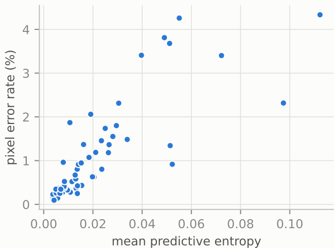
Per-image: entropy vs error ( r = 0.82 )
